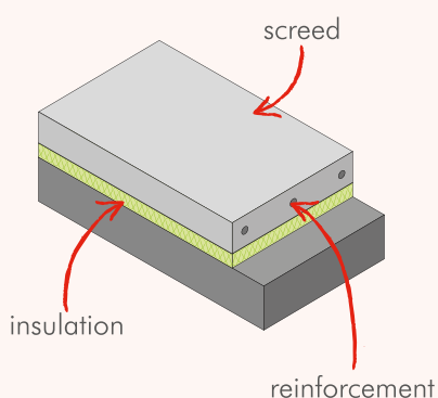
Floating Screed:
